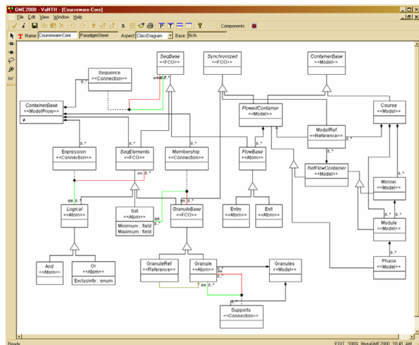
Figure 1: An Element of CAPE Meta-Design
