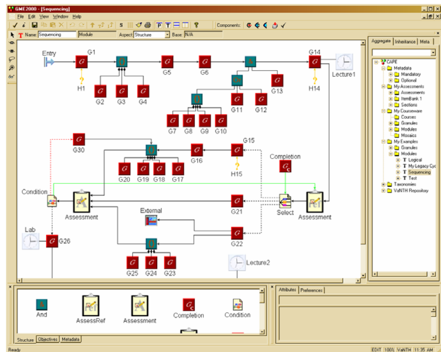
Figure 2: Delivery Sequencing in CAPE's Structure Aspect
