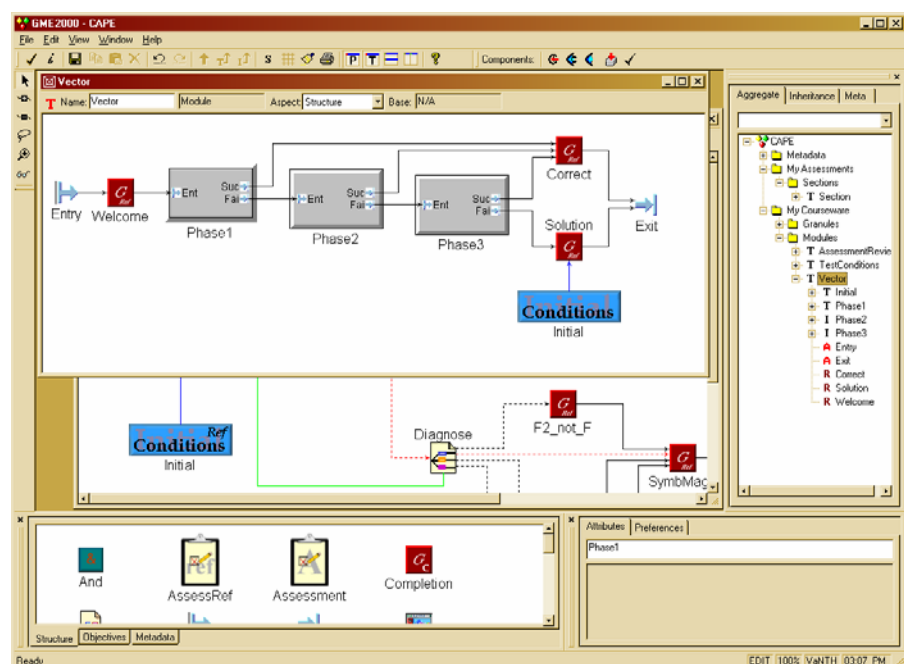
Figure 3: An Instructional Design Pattern for a Math Tutor
